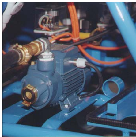
Water booster pump with automatic shut-off during breaks.
