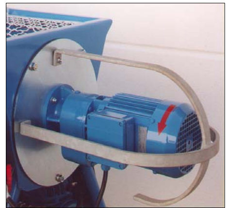
Quick disassembly of worm shaft motor by 3 nuts for transport and cleaning.
