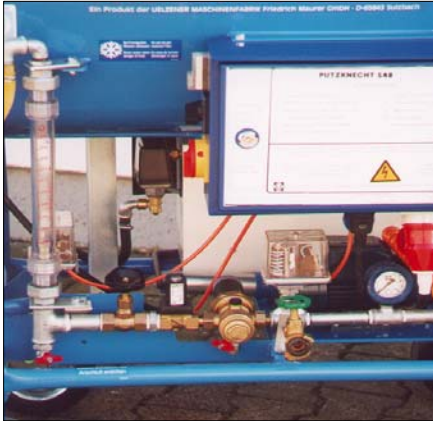
Compact water armature with integrated low pressure reducer.
