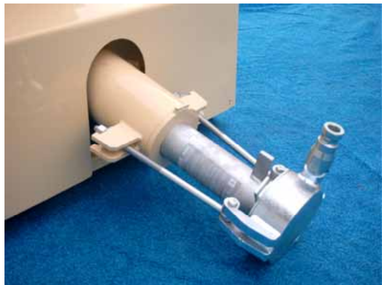
View to the worm pump, shown with re-mixer and pump outlet
